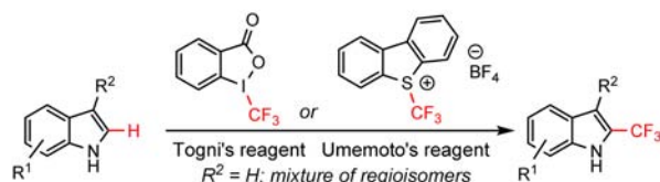
Scheme 1. Complementary Strategies for the Synthesis of 2-(Trifluoromethyl)indoles
