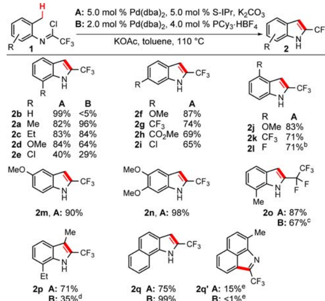
Scheme 2. 2-CF 3 -indoles Scope of the C(sp 3 )–H Functionalization a
